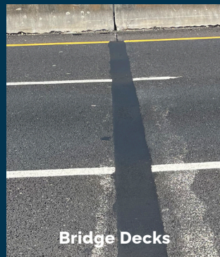
Wide Cracks
